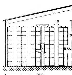
15 With stacker and reach fork-lift
